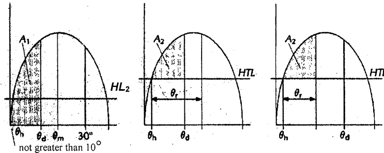
Figure 1 - Intact stability
