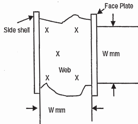
Figure 3 – Typical five-point pattern on the web plate
